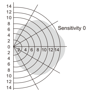
Wall Pattern (Unit: m) Installation Height: 2.5m
